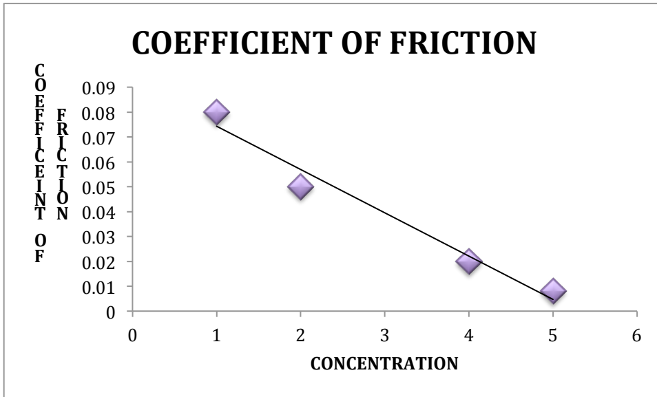
Figure 1. Graph displays performance data measured with lubricity tester. FRIC-SLICK'S coefficient of friction shows that this pipe on pipe lubricant will perform in challenging formations.
